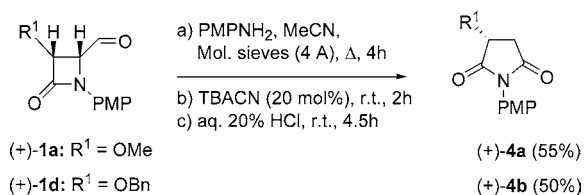
Scheme 3. One-Pot Synthesis of Succinimides 4 from \beta -Lactam Aldehydes 1
