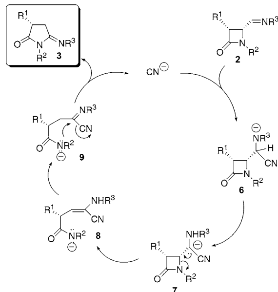
Scheme 2. Proposed Catalytic Cycle for the Formation of Succinimide Derivatives 3 from Imino- \beta -lactams 2
