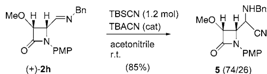
Scheme 1. Synthesis of \alpha -Amino Nitrile 5 from N -Benzylimino- \beta -lactam (+)- 2h
